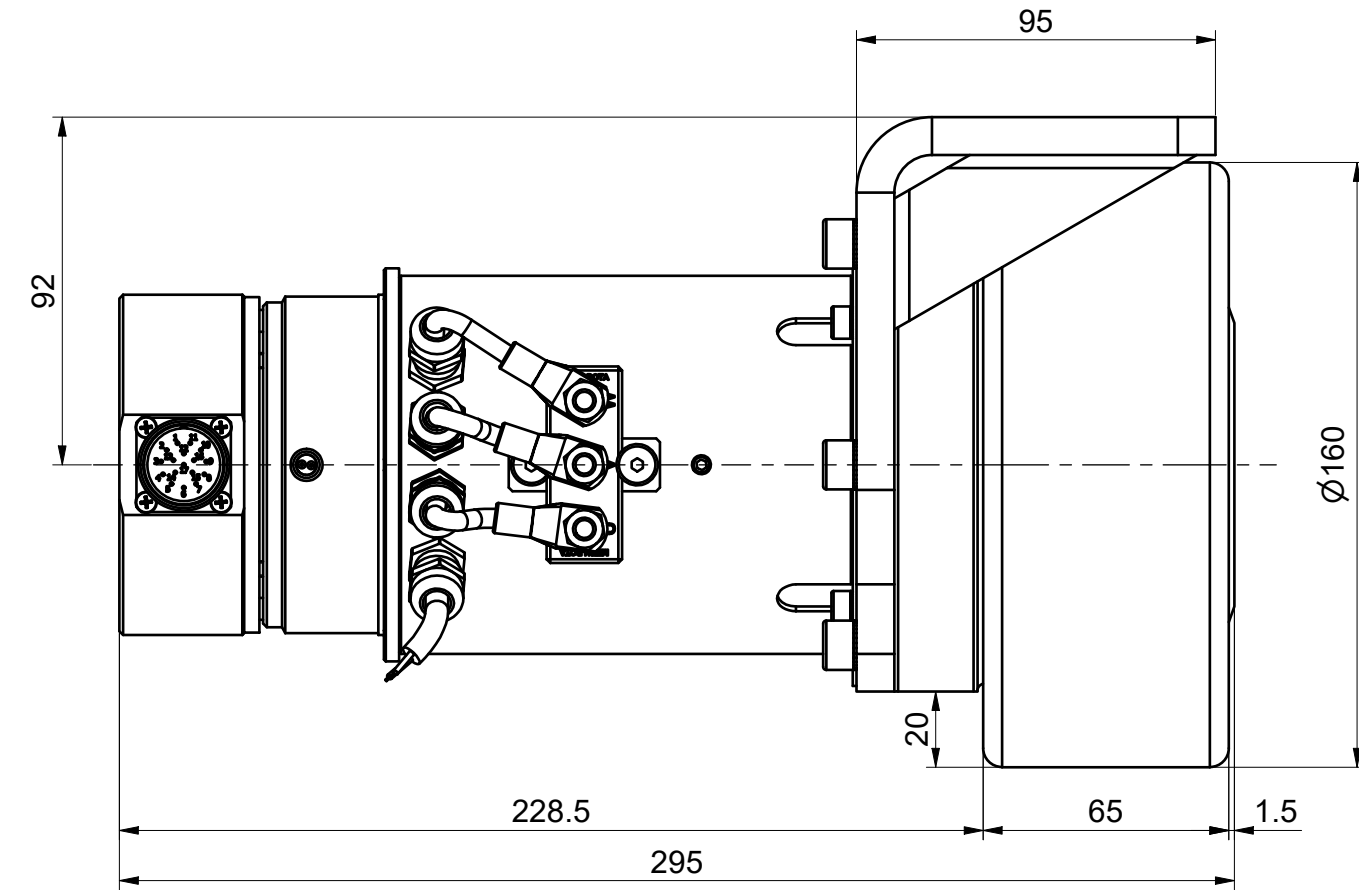
View with wheel and frame plate
