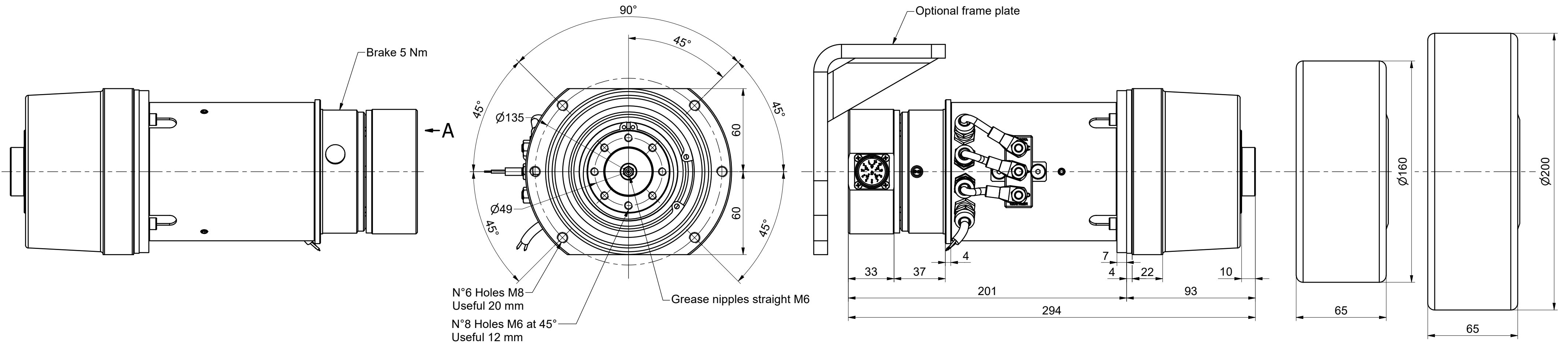
View from "A"
